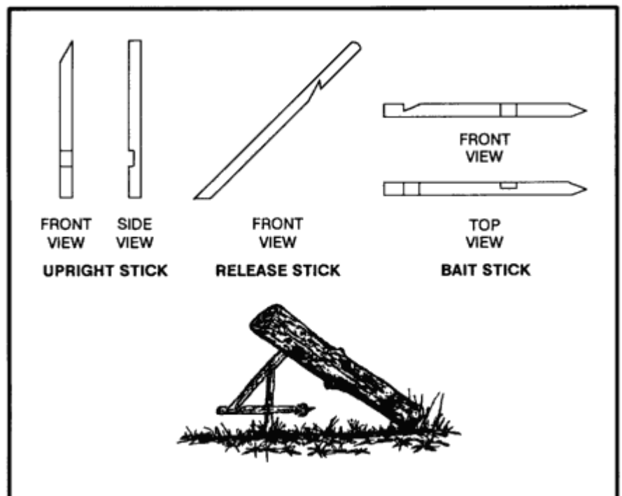
Figure 8-12. Figure 4 deadfall.
